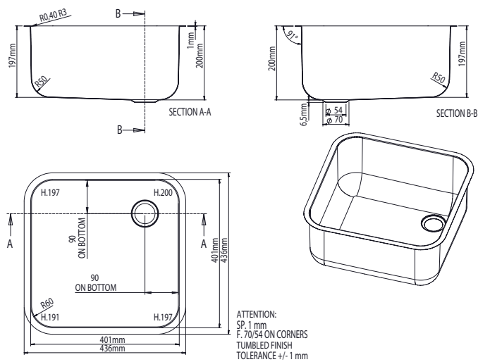
SBM-404020-TF
