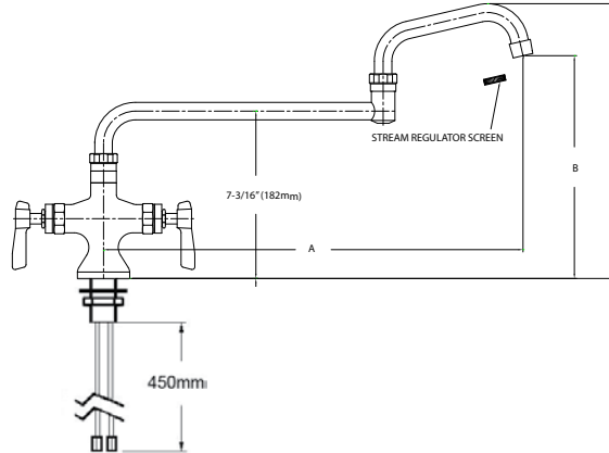
KL51-9xxx-SE1 Series
