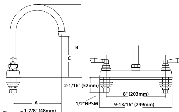
TLL11-81xx-SE1 Series
