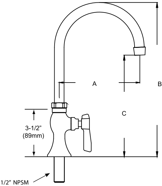
TLL20-9100x-SE1 Series
