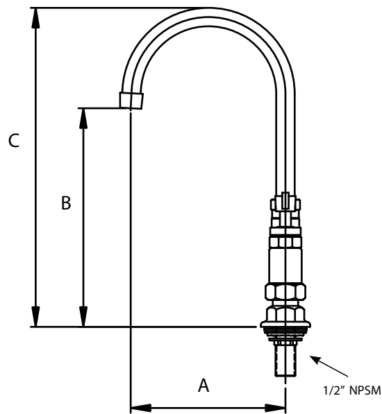
KL61-8x0x-xE2 Series
