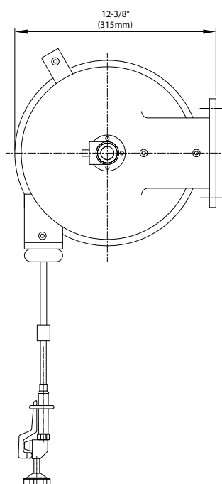
KHR-1015-OSS Series
