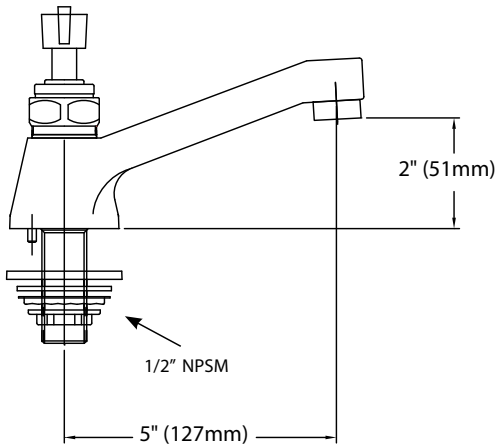
KL87-9105-xE1 Series
