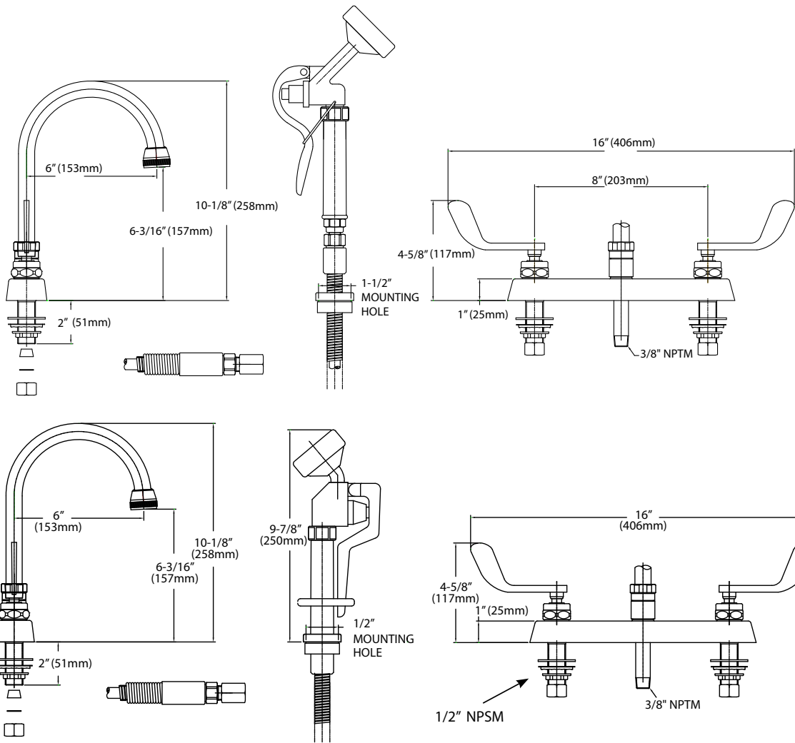
K41-8x01-724A Series
