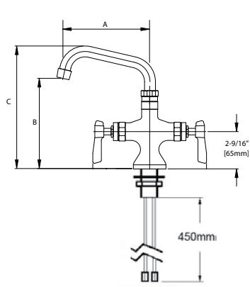
KL51-9xxx-SE1 Series
