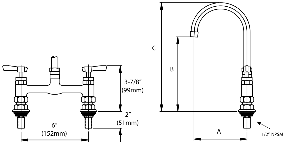
KL67-6x0x-xE1 Series
