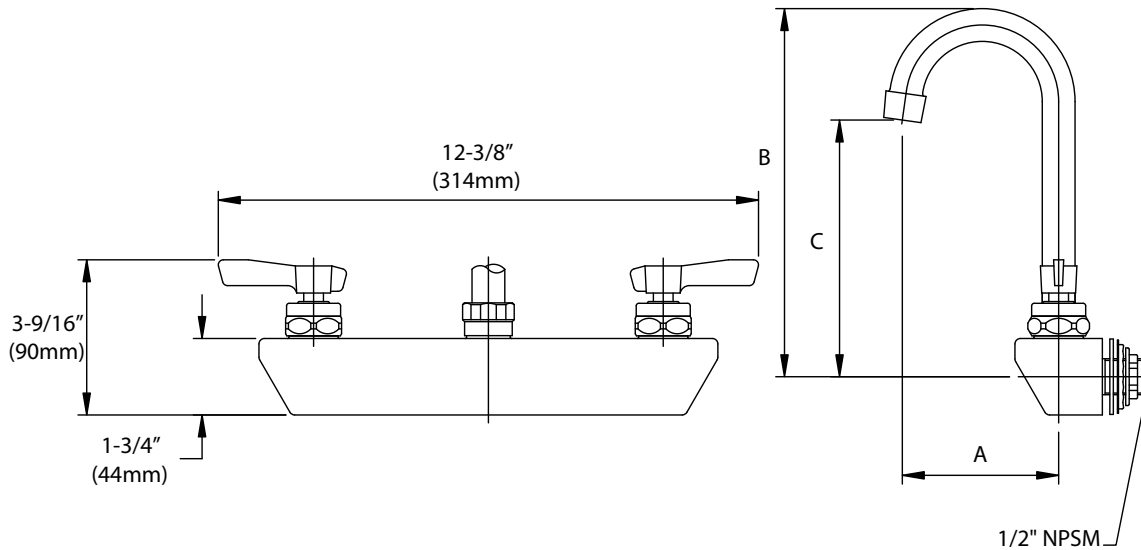
KL45-8x0x-xE1 Series
