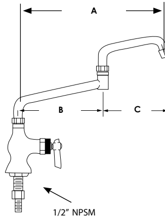
KL64-9xxx-SE1 Series
