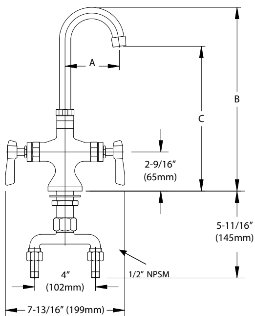
KL51-9x0x-xE2 Series
