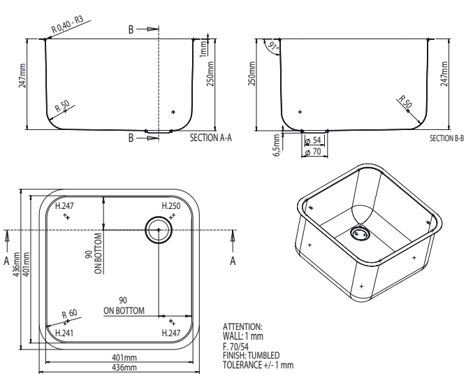
SBM-404025-TF
