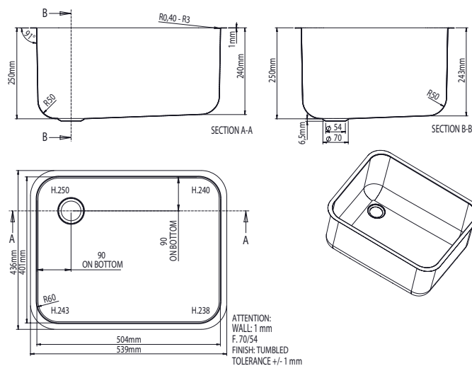
SBM-504025-TFL
