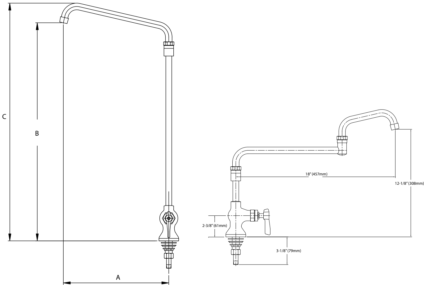
KL65-901x-SE1 Series
