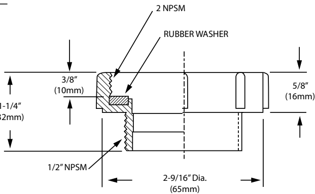
Reducer Assembly
