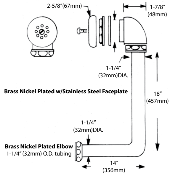
Overflow Assembly
