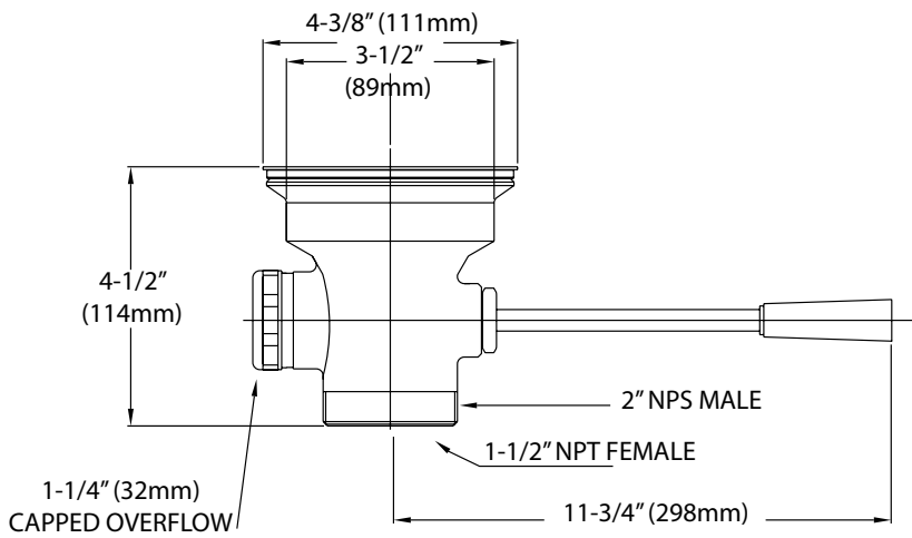
D15-751x Series
