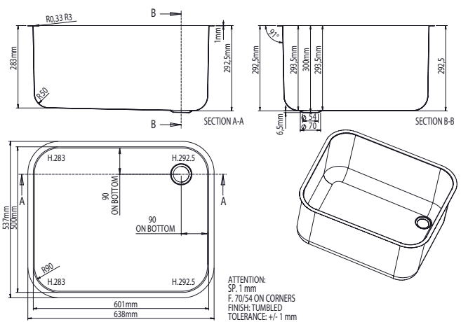
SBM-605030-TFR
