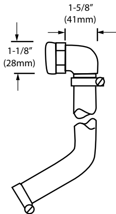
Overflow Assembly
