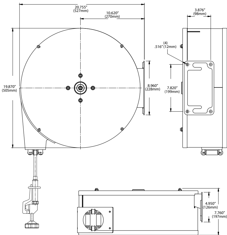
KHR-5650-E Series
