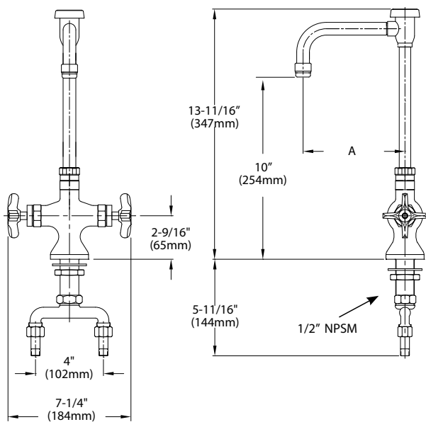
KN51-9x5x-KR1 Series
