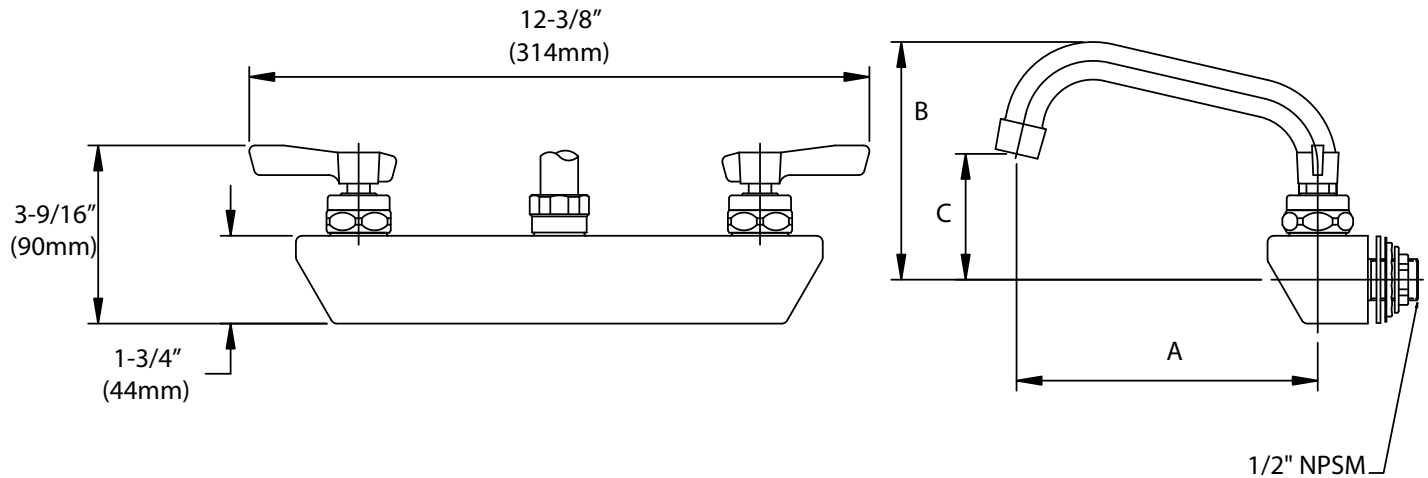
KL45-8xxx-xE1 Series
