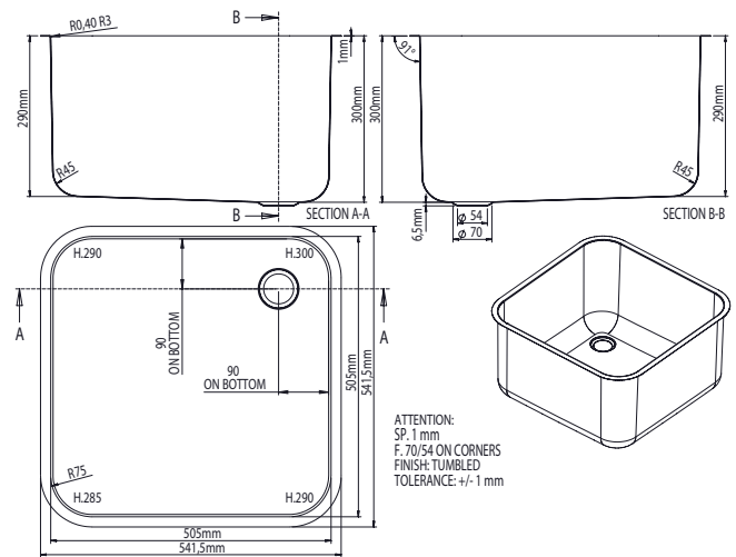
SBM-505030-TF
