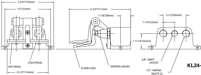
KL24-1100 Series
