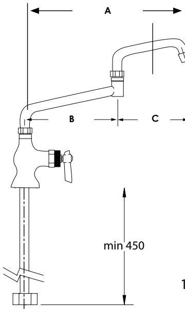
KL64-9xxx-SE1 Series
