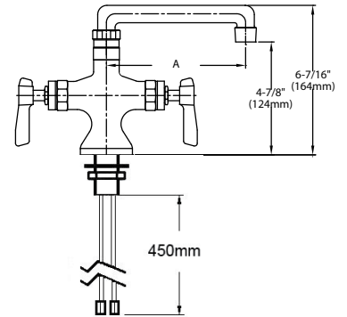
KL51-9x0x-TE1 Series
