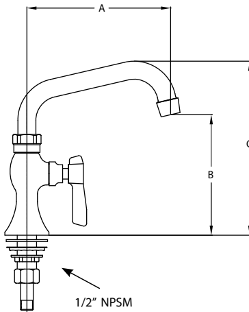
KL64-9x0x-SE1 Series
