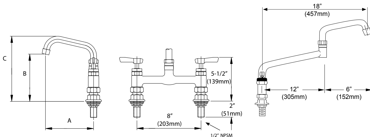
KL61-8xxx-SE1 Series
